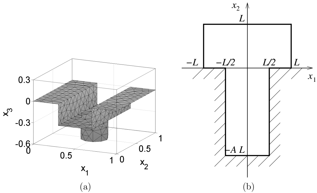
Figure 1: Schematics of (a) a three-dimensional trench-via structure (known as a ‘Damascene’ structure in industry) and (b) a two-dimensional trench defining the feature width L and aspect ratio A . Each plot shows the solid wafer surface. The gas domain of the KTRM is the region above the wafer surface up to the top of the plot box.
