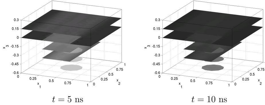
Figure 5: Slice plots of the dimensionless concentration c(\mathbf{x}, t) for \text{Kn} = 1.0 at heights x_3 = -0.60, -0.45, -0.30, -0.15, 0.00, 0.15 at different times. Grayscale from light \Leftrightarrow c = 0 to dark \Leftrightarrow c = 1 .
