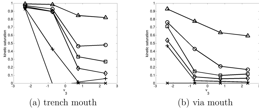
Figure 6: Line plots of the saturation of the kinetic density f(\mathbf{x}, \mathbf{v}, t)/M(\mathbf{v}) for \text{Kn} = 1.0 for v_1 = v_2 = 0 as a function of v_3 ; (a) at the mouth of the trench at position \mathbf{x} = (0.5, 0.5, 0.0) and (b) at the mouth of the via at position \mathbf{x} = (0.5, 0.5, -0.3) ; at times: \times = 1 ns, + = 2 ns, \diamond = 3 ns, \square = 4 ns, \circ = 5 ns, \triangle = 10 ns.
