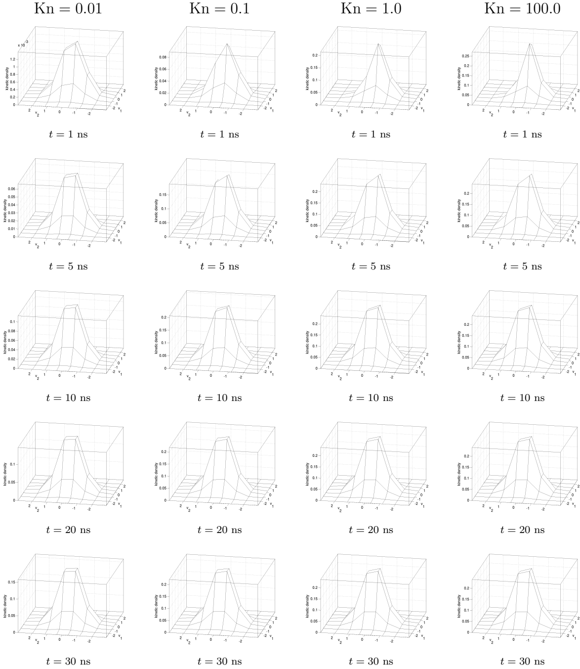
Figure 3: Dimensionless kinetic density f(\mathbf{x}, \mathbf{v}, t) as a function of \mathbf{v} \in \mathbb{R}^2 at \mathbf{x} = (0.0625, 0.0) in the two-dimensional trench for selected Knudsen numbers Kn at selected times. Notice the different scales on the vertical axes in some plots.
