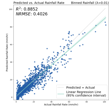
Fig. 5. Results from using the model generated from a binned rainfall loss term ( \lambda = 0.01 ).
