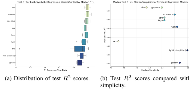
Fig. 3. Accuracy and simplicity of symbolic regression models.
