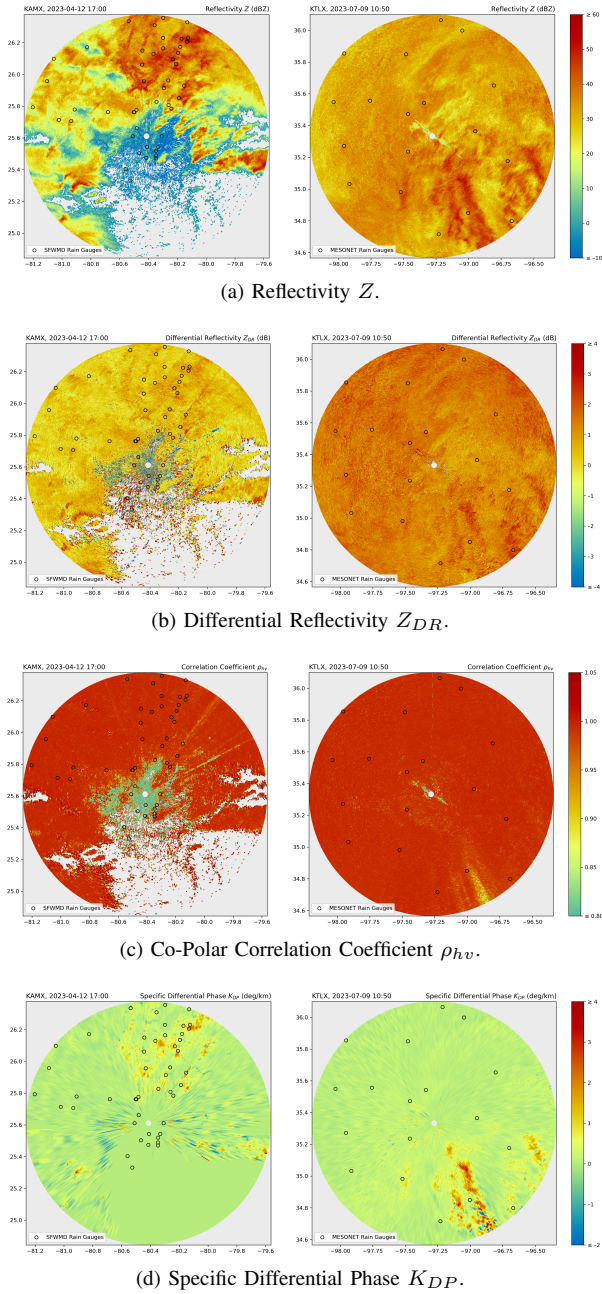
Fig. 1. WSR-88D radar data of rainfall events in South Florida (KAMX) and Central Oklahoma (KTLX).
