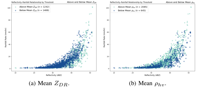
Fig. 2. Reflectivity-rainfall relationship for above and below mean Z_{DR} and mean \rho_{hv} .
