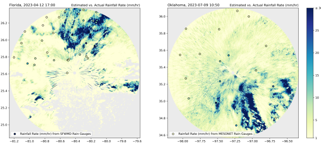
Fig. 4. Estimated rainfall rate from RILS-ROLS equation (Table IV) compared with actual rainfall rate from rain gauges.
