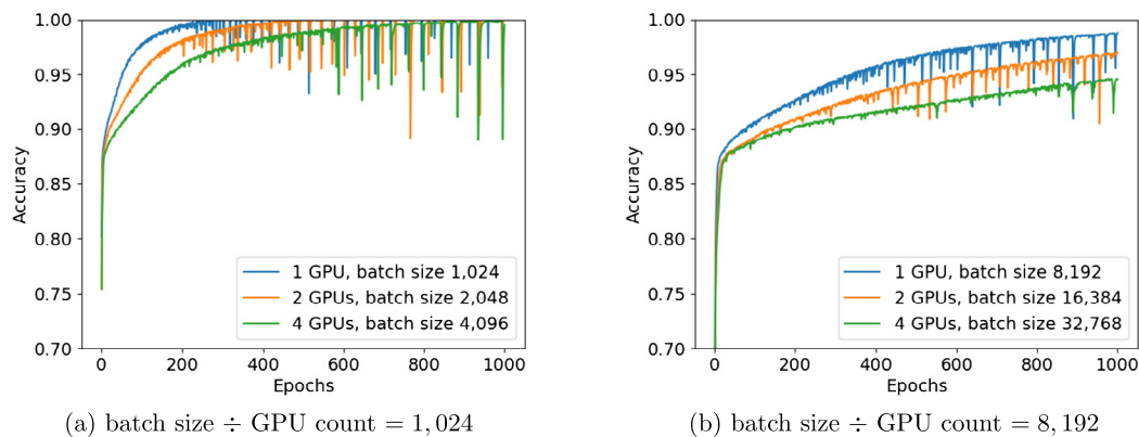
Fig. 8. Training accuracy curves varied by both GPUs and batch size simultaneously, with data multiplier 1 and learning rate 0.001 for the 2018 GPUs with preaugmented data and forced parallelism.
