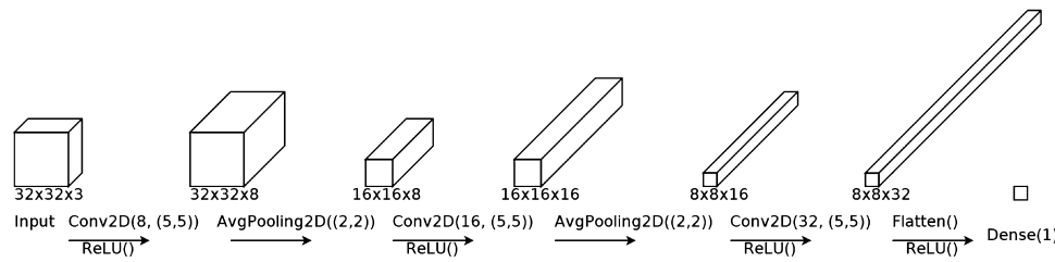
Fig. 1. The structure for the convolutional neural network used for tornado prediction.
